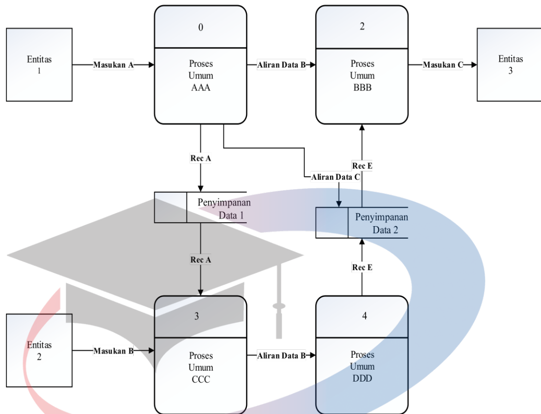
Gambar 2. 6 Contoh Diagram Level 0
