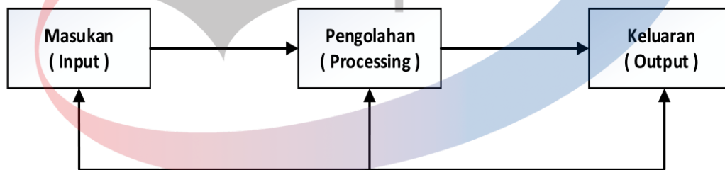
Gambar 2. 1 Model Sistem
